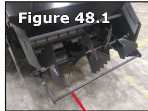
SAFETY BAR REMOVE COTTER PIN ON BOTH ENDS OF SAFETY BAR
