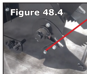
REMOVE THIS NUT, LOCKWASHER AND BOLT. THE LOCKWASHER AND NUT WILL BE USED LATER
